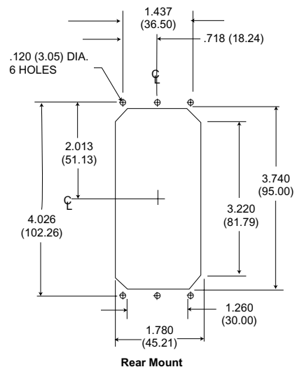
Rear Mount
