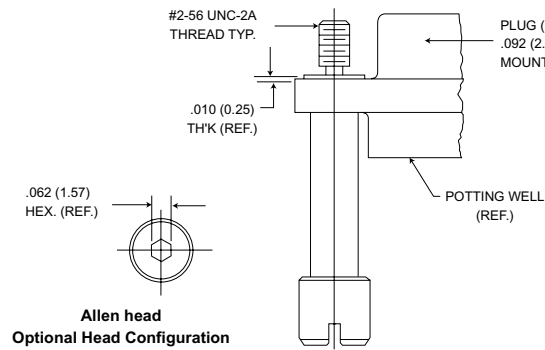
Jackscrew - (K) High Profile Slotted Head
