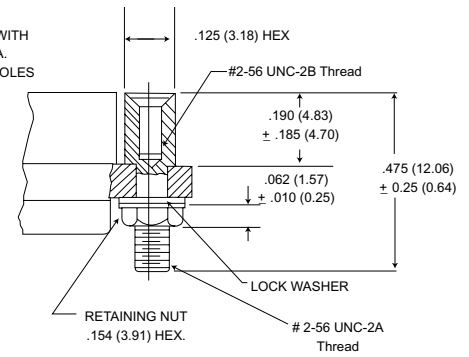
Jackpost Assembly
