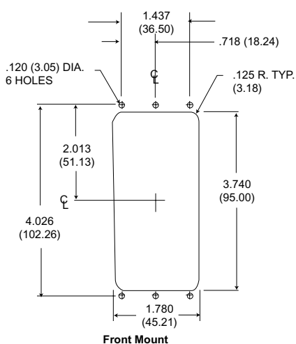
Front Mount
