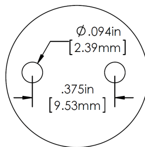
PCB HOLE SIZE AND CENTER TO CENTER SPACING
