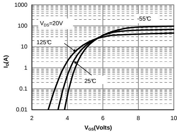
Figure 3: Transfer Characteristics
