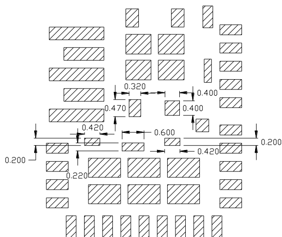
SOLDER PASTE STENCIL PAD SIZES (DETAIL 2)
