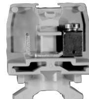
Channel Mount (Dovetail Base)
