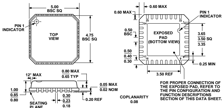
COMPLIANT TO JEDEC STANDARDS MO-220-VHHD-2 Figure 75. 32-Lead Lead Frame Chip Scale Package [LFCSP_VQ] 5 mm x 5 mm Body, Very Thin Quad (CP-32-4) Dimensions shown in millimeters
