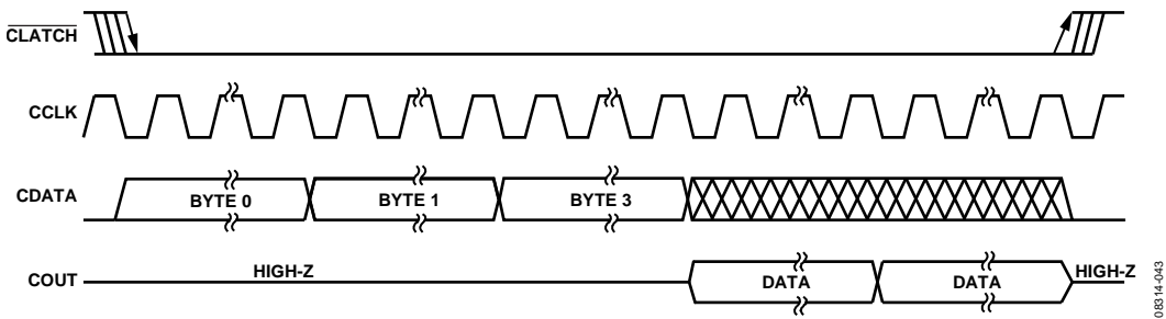
Figure 44. SPI Read from ADAU1781 Clocking (Single-Read Mode)
