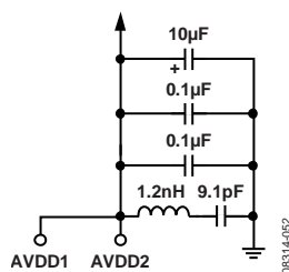
Figure 56. GSM Filter on the Analog Supply Pins
