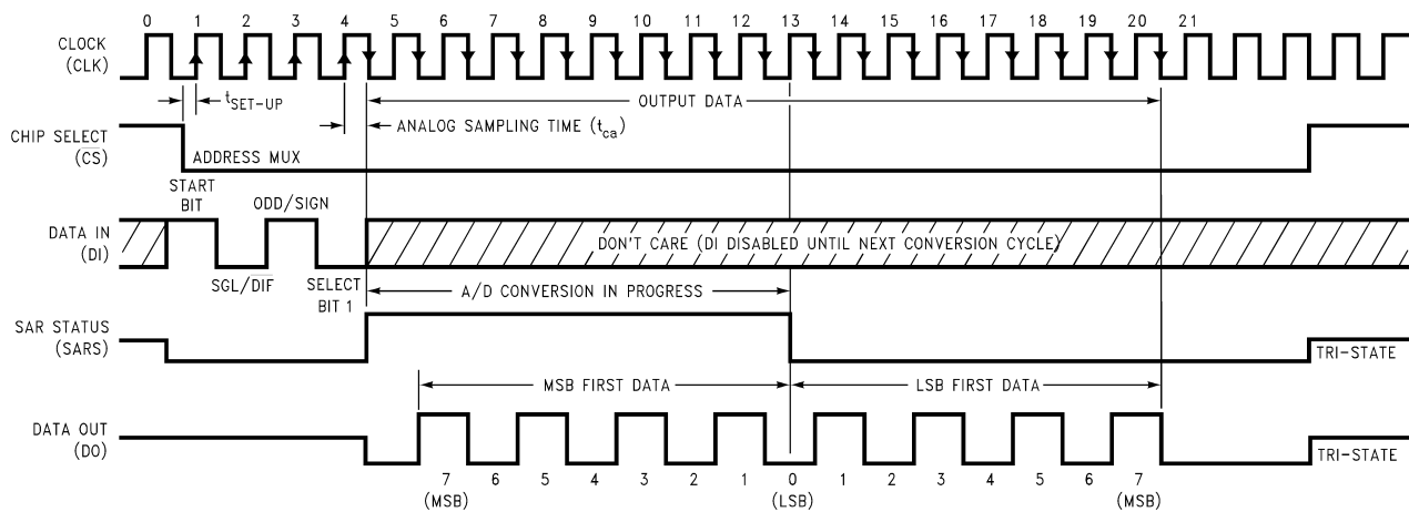
Figure 18. ADC08038 Timing
