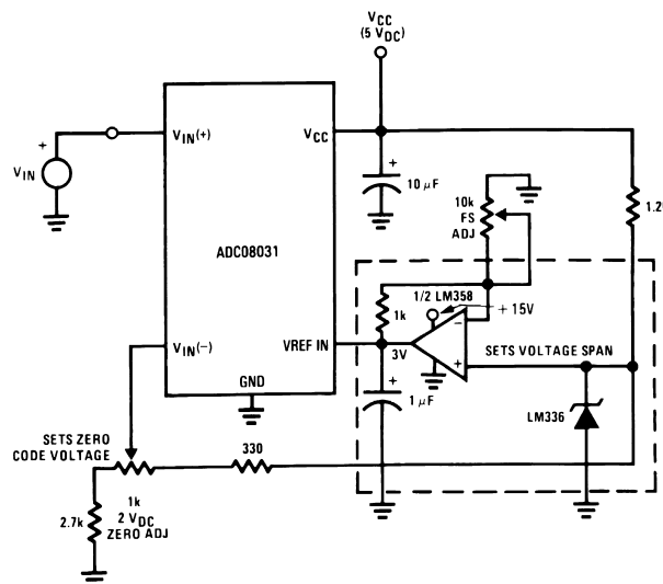
Figure 26. Zero-Shift and Span Adjust: 2V \leq V_{IN} \leq 5V
