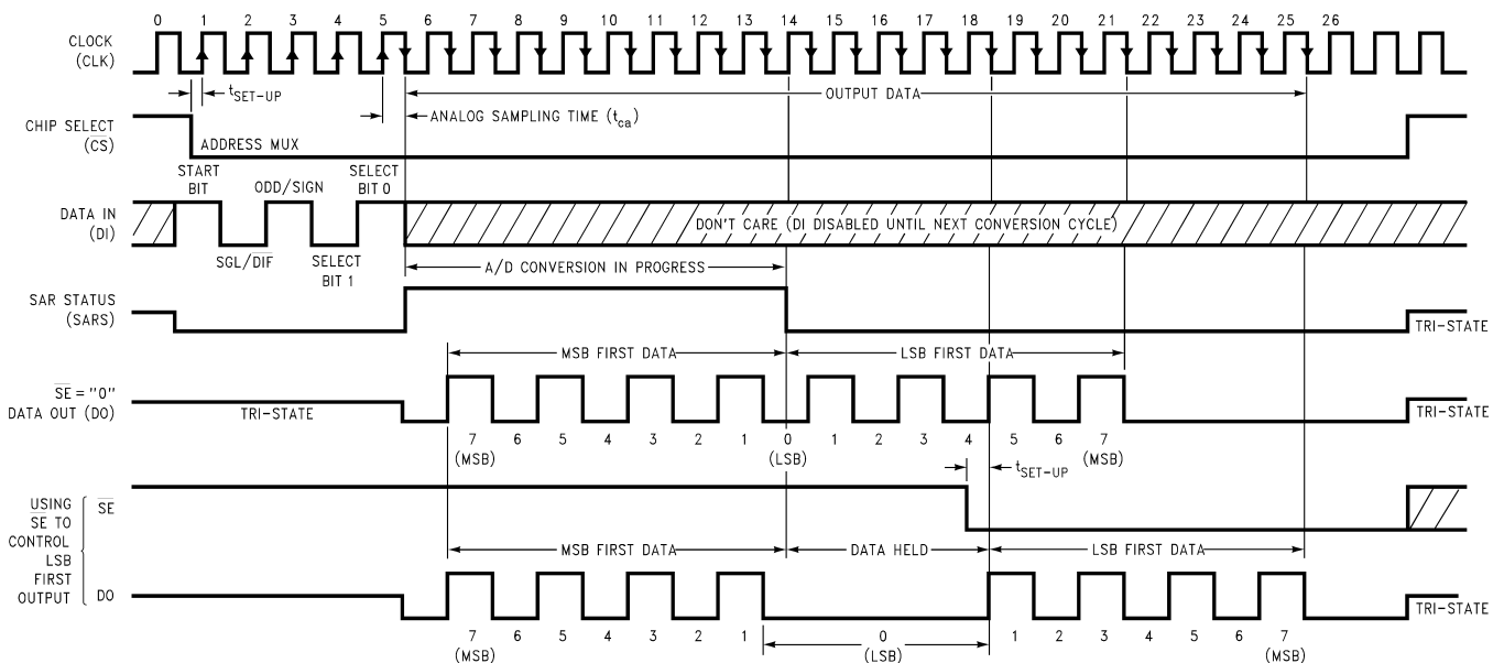
Figure 18. ADC08038 Timing
