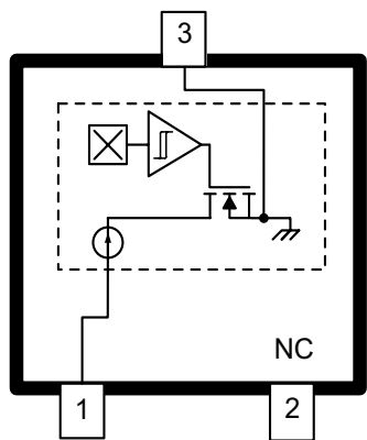
LH Package, 3-Pin SOT23W Pinout
