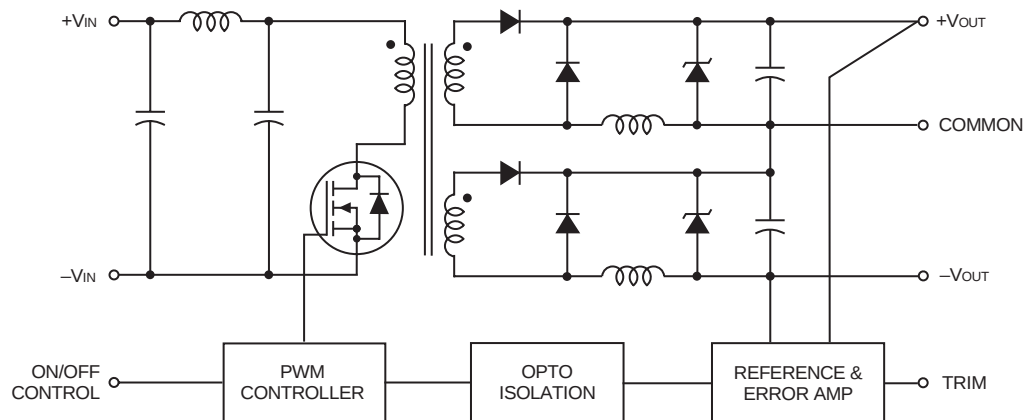
Figure 1. Simplified Schematic
