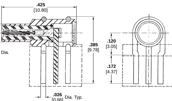
Right-Angle Printed Circuit Receptacle Mounting Hole Pattern Shown Below Part Number 141-1005-0001
