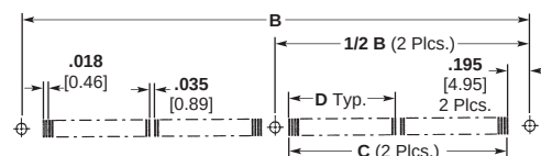
Size 304 & 400 Recommended PCB Footprint Pattern
