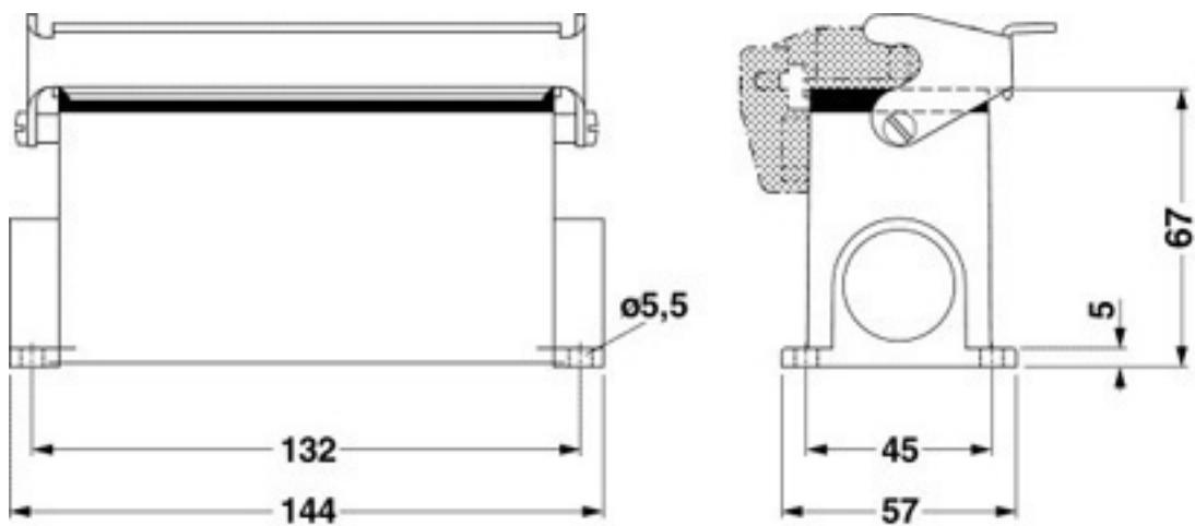
Dimensioned drawing
