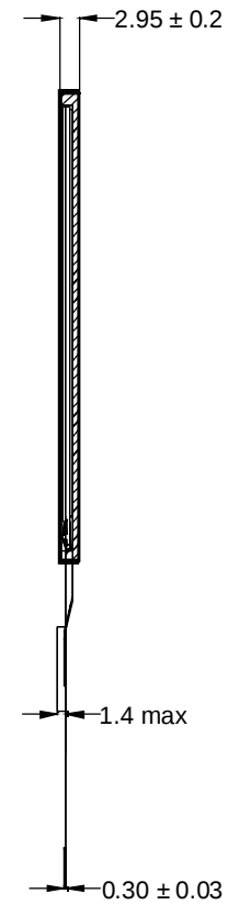
Side View (TFT)
