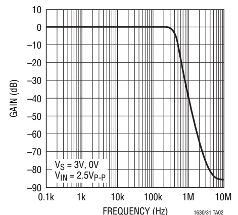
Frequency Response
