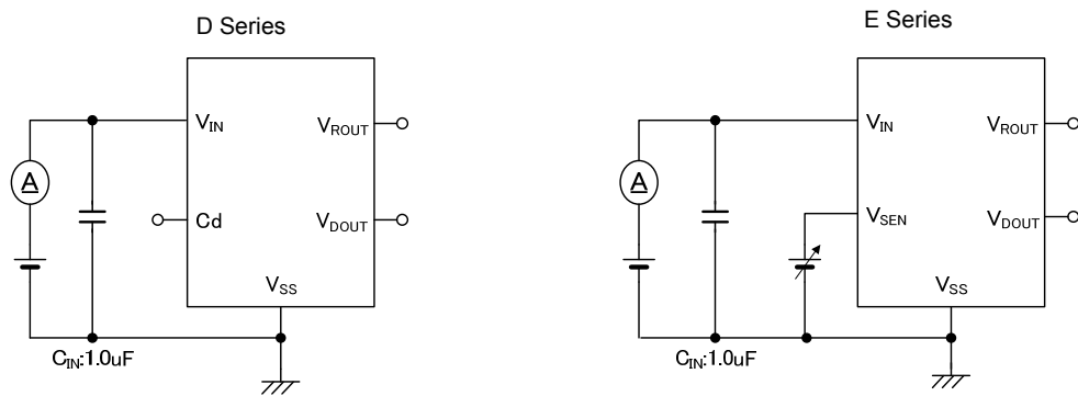
Circuit ②
