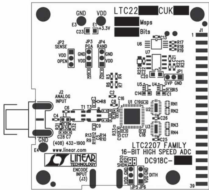
Silkscreen Top
