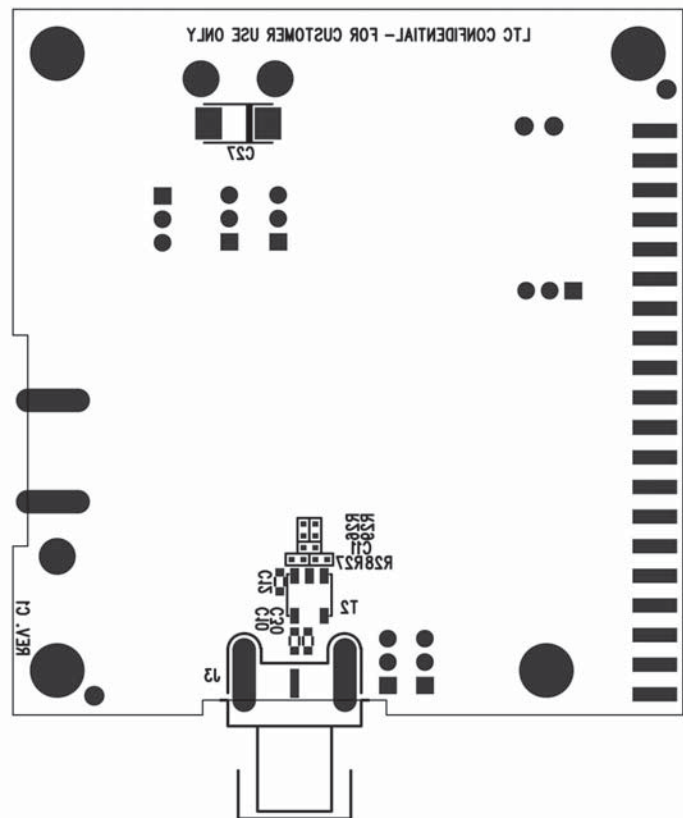
Silkscreen Bottom
