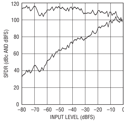
LTC2207-14: SFDR vs Input Level, f_{IN} = 15.1\text{MHz} , \text{PGA} = 0 , \text{RAND} "On", Dither "Off"
