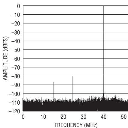
LTC2207-14: 32K Point FFT, f_{IN} = 250.1\text{MHz} , -1\text{dBFS} , PGA = 1, RAND "On", Dither "Off"
