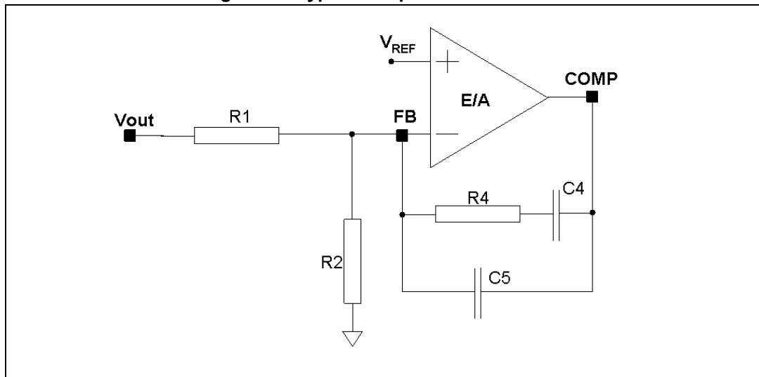
Figure 14. Type II compensation network
