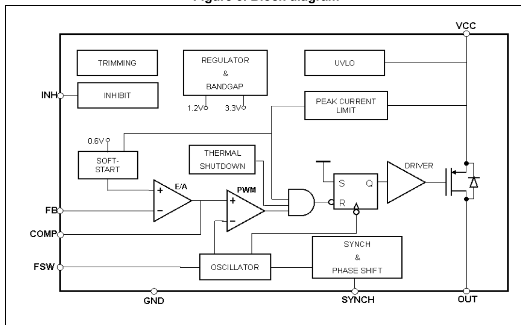
Figure 3. Block diagram
