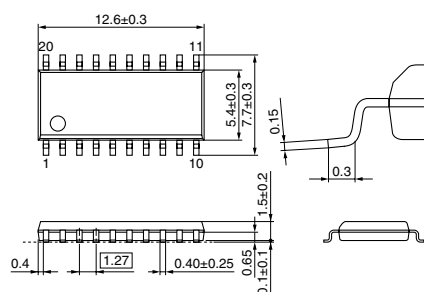
SOP020-P-0300B
