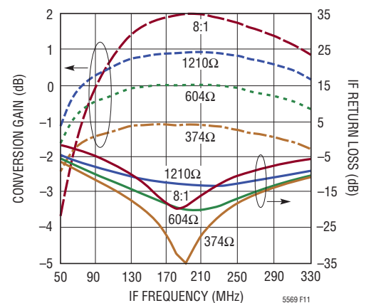
Figure 11. Conversion Gain and IF Output Return Loss vs IF Frequency—Wideband Matching with 4:1 Transformer
