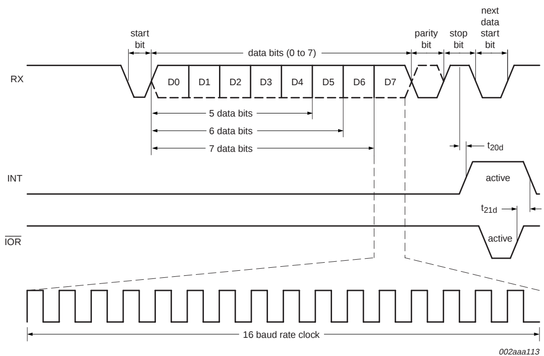
Fig 19. Receive timing
