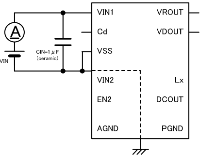
Circuit No.2
