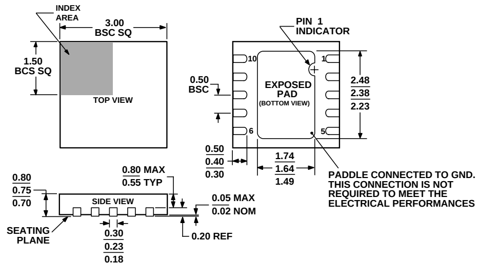
Figure 50. 10-Lead Lead Frame Chip Scale Package [QFN¹ (LFCSP_WD)] 3 mm × 3 mm Body, Very Very Thin, Dual Lead (CP-10-9)
