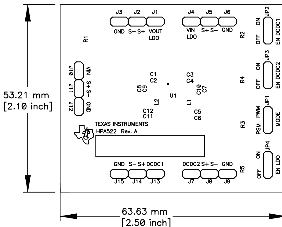
Figure 4. TPS657051/2EVM Silkscreen Top, X-Ray View
