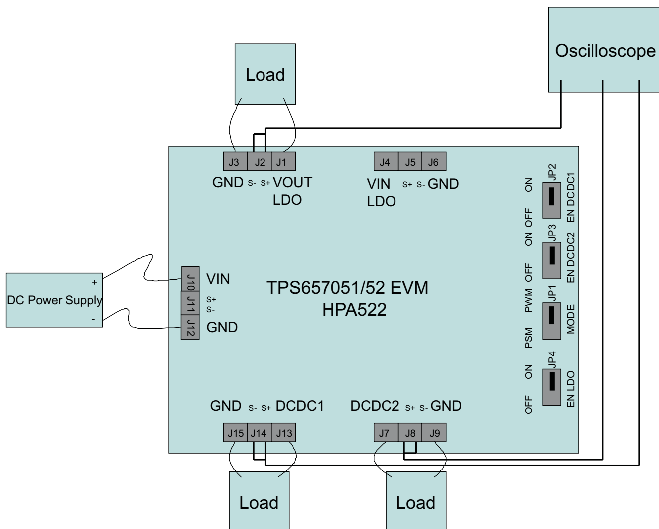
Figure 2. Hardware Board Connection
