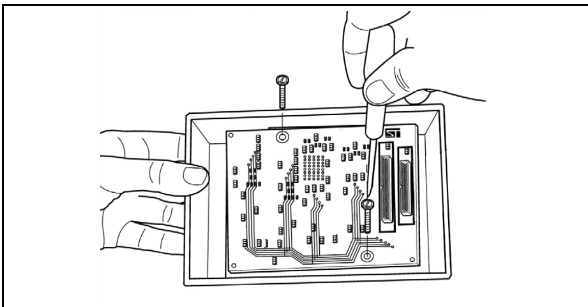
Figure 9: Removing the TEB screws
