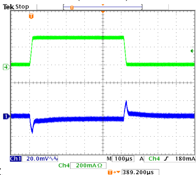
LOAD TRANSIENT RESPONSE (1mA to 300mA)
