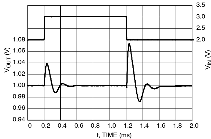
Figure 43. Line Transients, 1.0 V Version, t_R = t_F = 5 \mu s , I_{OUT} = 1 mA , AE = 0 V
