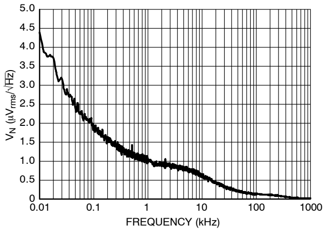
Figure 41. Output Voltage Noise, 1.8 V Version, V_{IN} = 2.8 V , I_{OUT} = 30 mA
