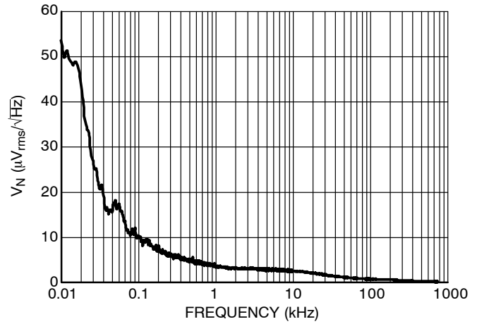
Figure 40. Output Voltage Noise, 1.2 V Version, V_{IN} = 2.2 V , I_{OUT} = 30 mA
