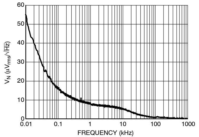
Figure 42. Output Voltage Noise, 3.3 V Version, V_{IN} = 4.3 V , I_{OUT} = 30 mA
