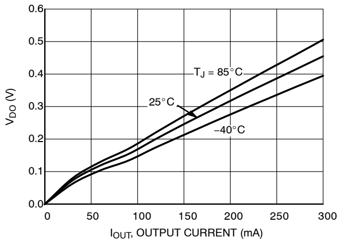
Figure 7. Dropout Voltage vs. Output Current 1.0 V Version
