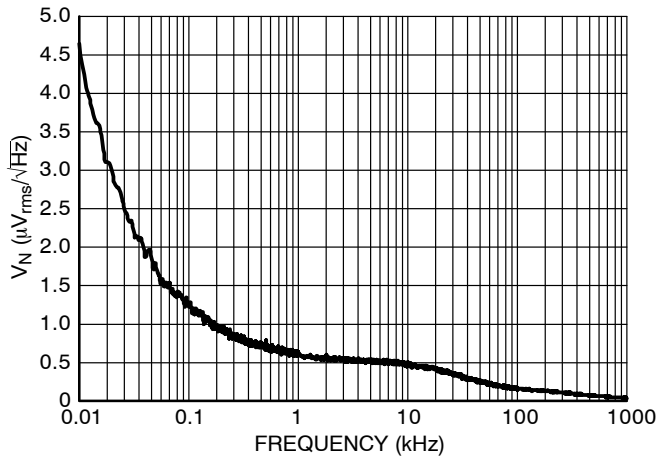
Figure 39. Output Voltage Noise, 1.0 V Version, V_{IN} = 2.0 V , I_{OUT} = 30 mA
