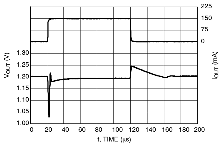
Figure 61. Load Transients, 1.2 V Version, I_{OUT} = 1 - 150 \text{ mA} , t_R = t_F = 0.5 \mu\text{s} , V_{IN} = 2.2 \text{ V} , AE = 0 \text{ V}
