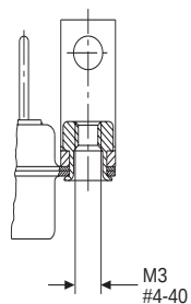
Metal Bracket with Captive Nut (1A9N/1A7N) (M3/4-40)
