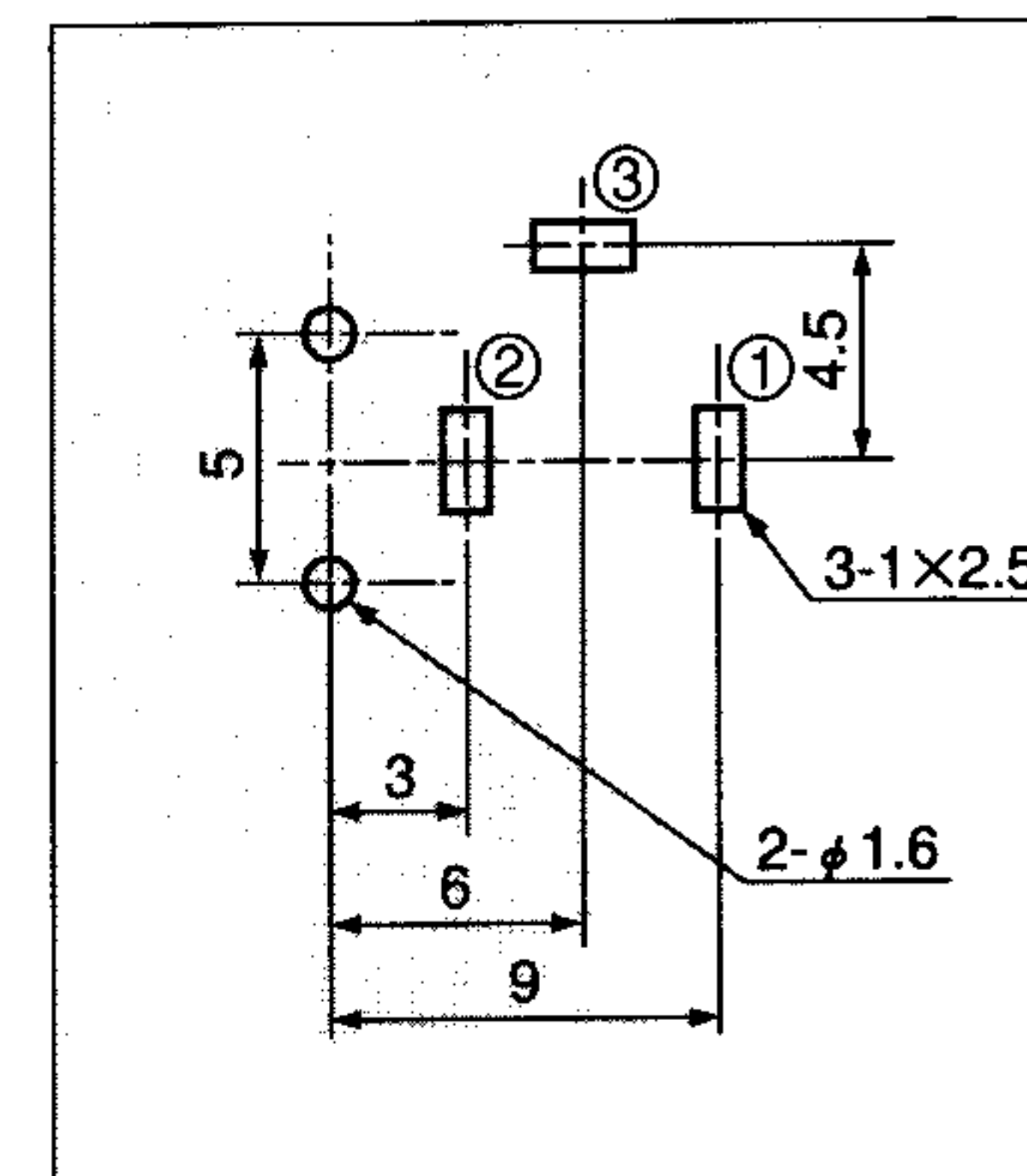
HOLE LAYOUT (BOTTOM VIEW)
