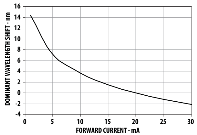
Figure 4. Relative Dominant Wavelength vs Forward Current
