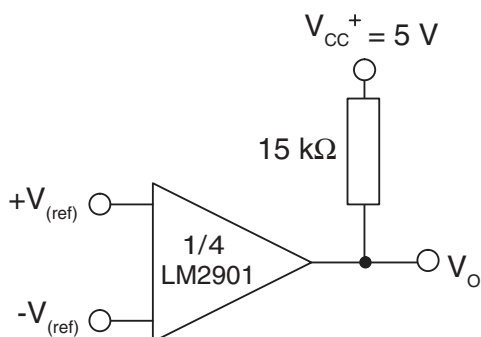
Figure 8. Basic comparator
