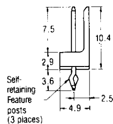
Section X-X
