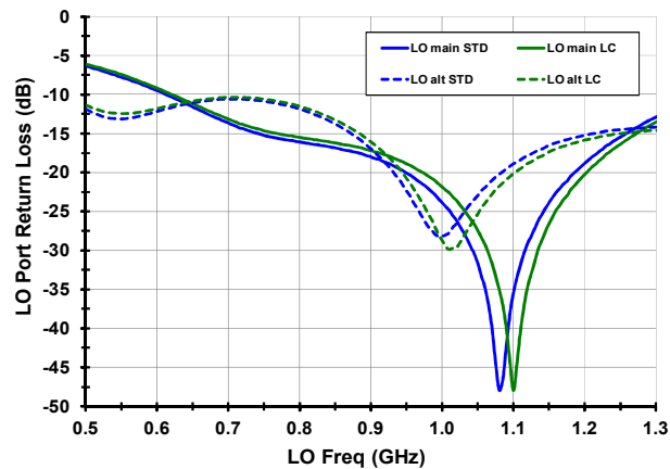
EVkit LO Port Match ( T_A = 25^\circ\text{C} , P_{MEAS} = 0 dBm)
