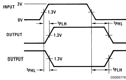
FIGURE 2. Propagation Delays
