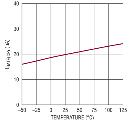
Gate Current (Charge Pump On) vs Temperature
