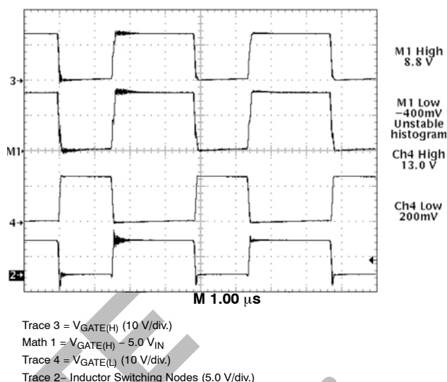
Figure 20. CS5161/5161H Gate Drive Waveforms Depicting Rail to Rail Swing
