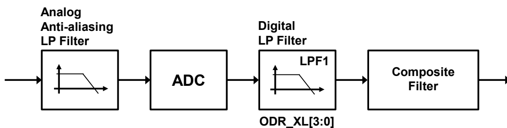
Figure 16. Accelerometer UI chain
