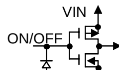
Figure 8 ON/OFF Pin
