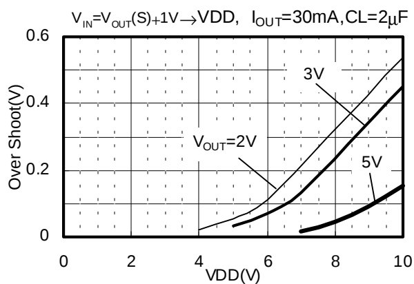
VDD dependence of overshoot
