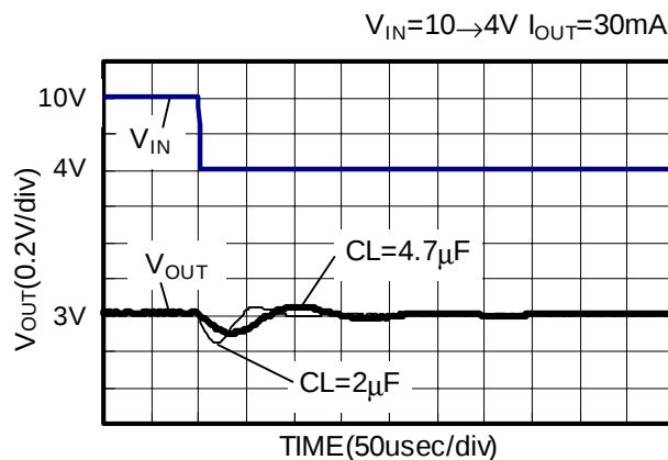
Output capacitor (CL) dependence of overshoot
