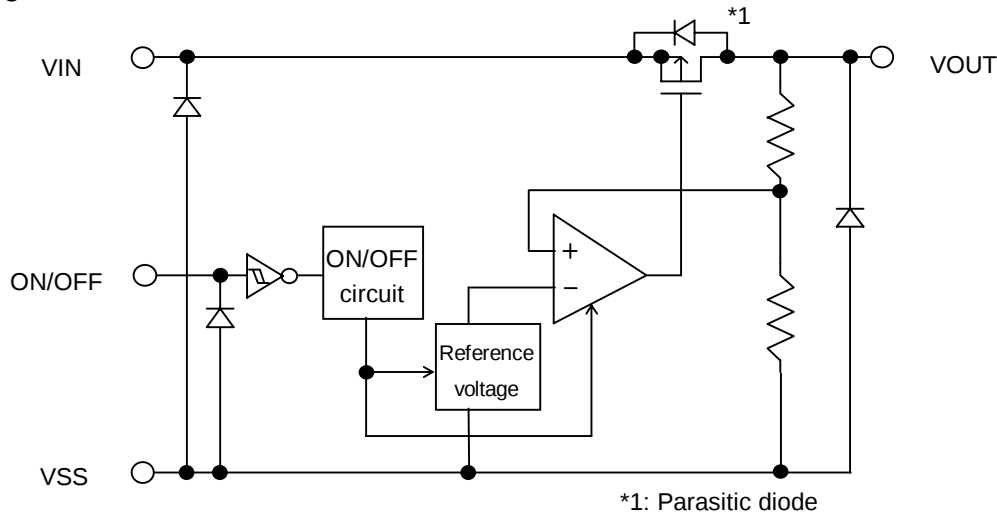
Figure 1 Block Diagram
