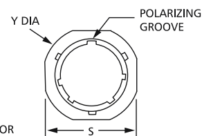
RECEPTACLE ASSEMBLY
