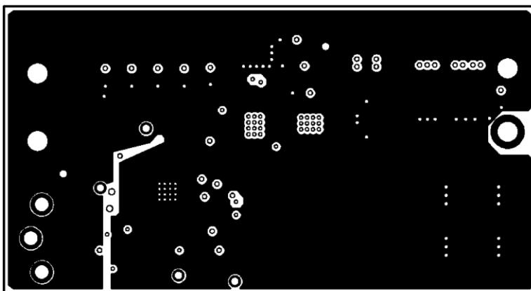
LAYER 2 (LY2) AS VIEWED FROM TOP
