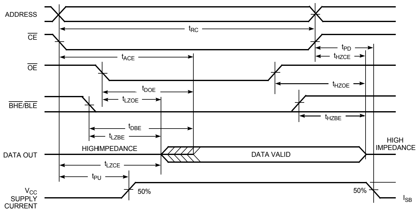
Figure 6. Read Cycle 2: \overline{\text{OE}} Controlled [22, 23]
