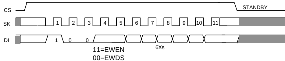
Figure 21 EWEN/EWDS Timing (S-93C66A)
