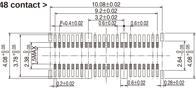
< 48 contact >
