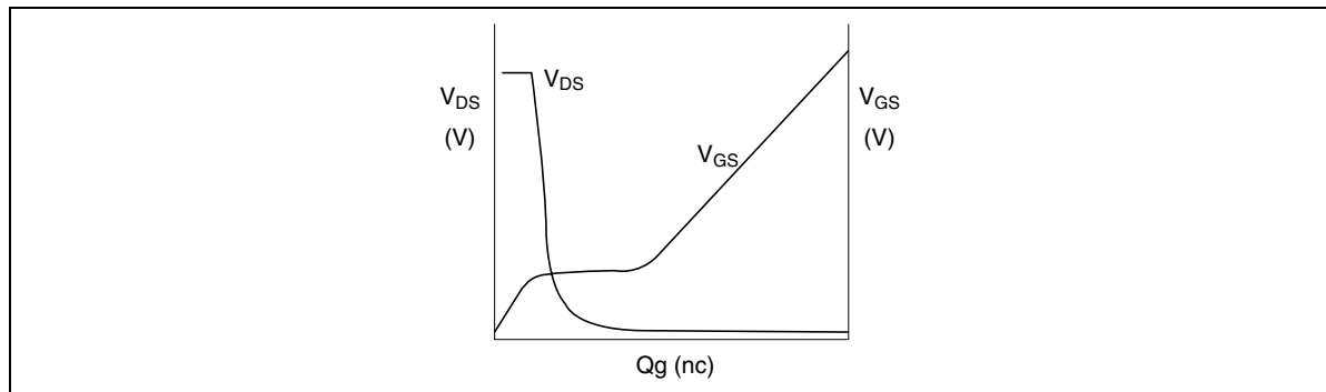
Figure 4.2 Power MOS FET Dynamic Input Characteristics
