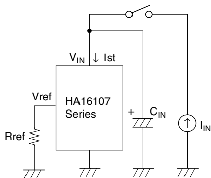
Figure 1 Standby Current Test Circuit
