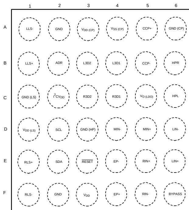
Figure 2. DSBGA Package See Package Number YPG0036CCA
