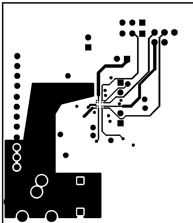
Figure 56. Layer 2
