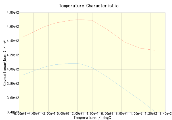
C2012X7R1E474K125AA(DC Bias = 0V) C2012X7R1E474K125AA(DC Bias = 12.5V)
