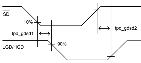
Figure 6. \overline{SD} Propagation Delay Timing for IXS839A/B
