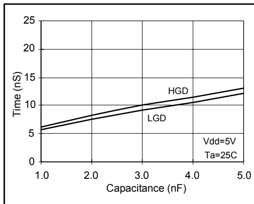
Fig 12. HGD and LGD Fall Time vs. Load Capacitance
