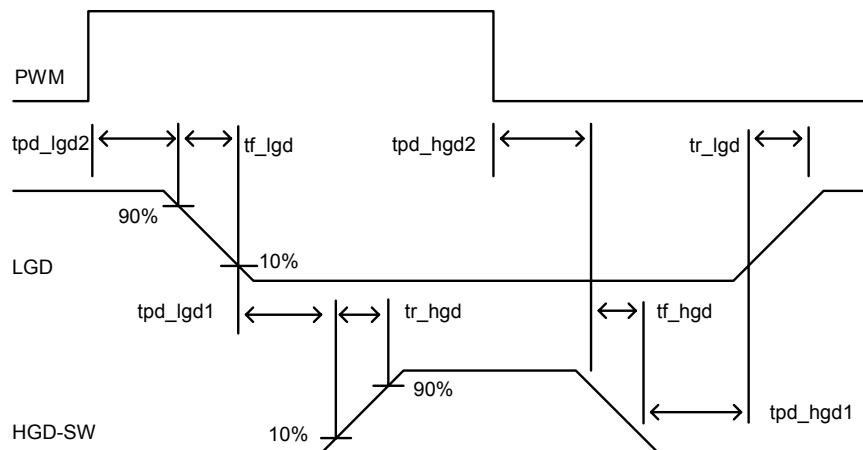
Figure 4. Non-Overlap Timing Diagram for IXS839/839A/839B
