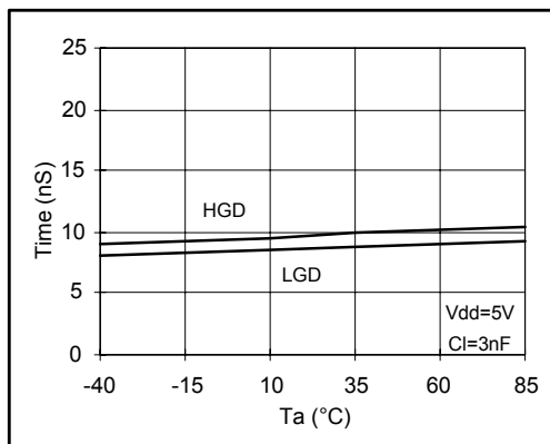
Fig 10. HGD &amp; LGD Fall Time vs. Temperature
