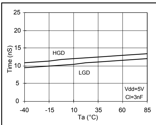
Fig 9. HGD &amp; LGD Rise Time vs. Temperature
