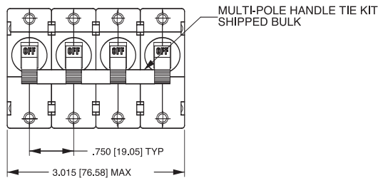
4-POLE (AB4)
