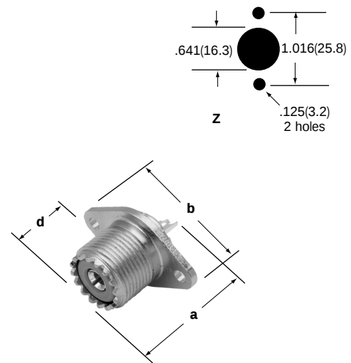
Panel Receptacle, 2 Hole Flange 83-876
