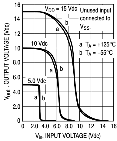
Figure 3. Typical Voltage Transfer Characteristics versus Temperature
