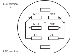
Contact Layout
