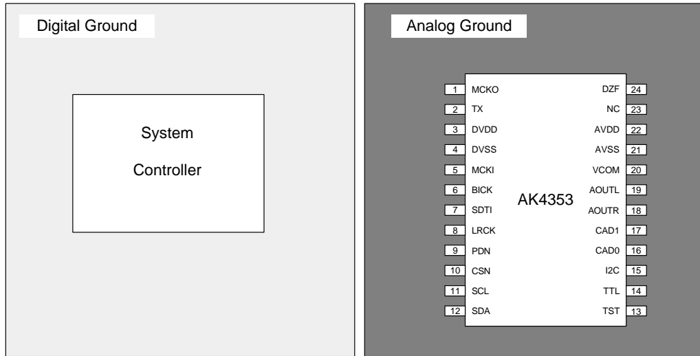
Figure 14. Ground Layout
