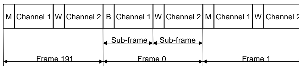
Figure 6. Block format
